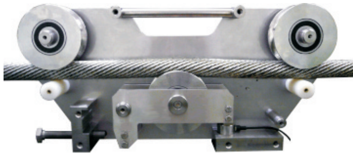
Foto: KSW 3-R with side plate dismounted
