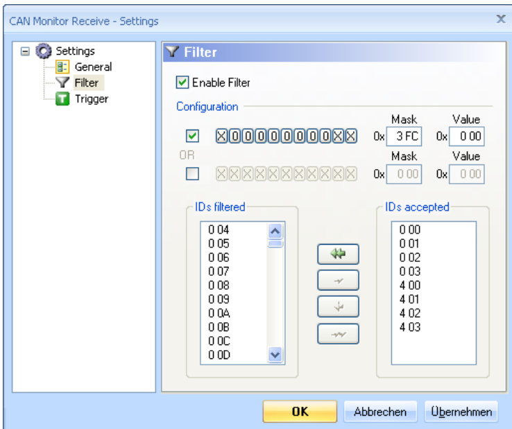
Figure 21: CAN Monitor Receive: Filter options
