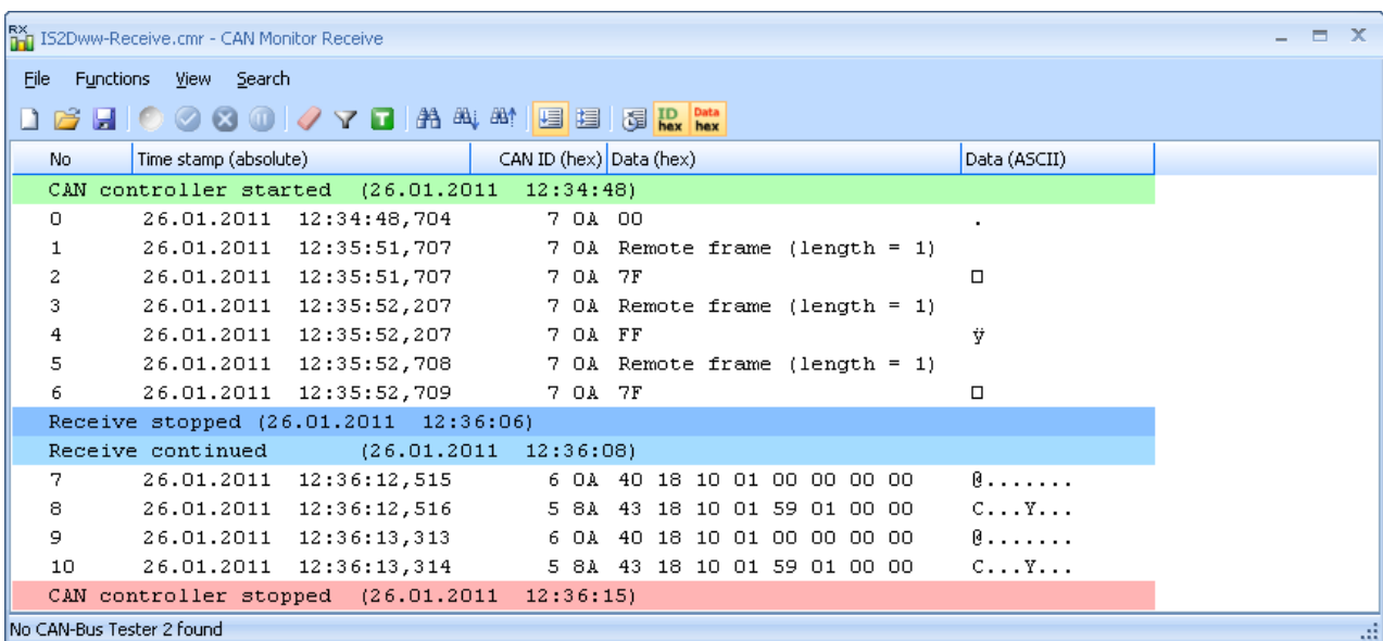
Figure 19: CAN Monitor Receive; “Scroll” mode
