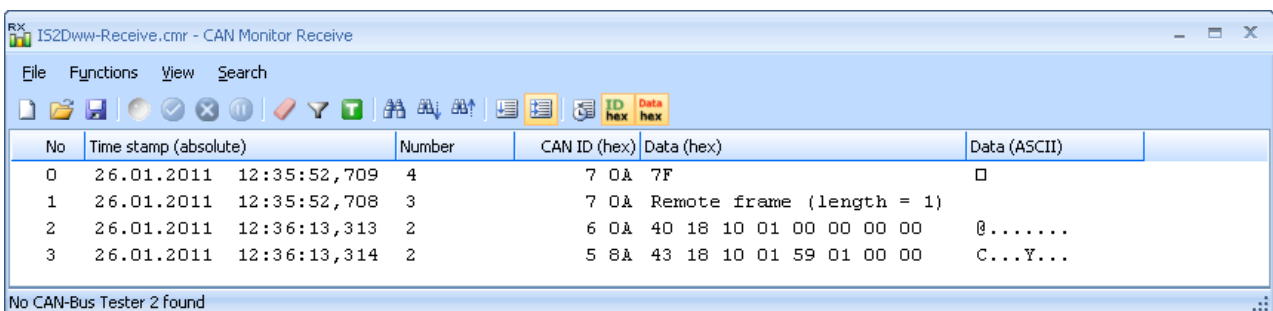
Figure 20: CAN Monitor Receive; “Overwrite” mode
