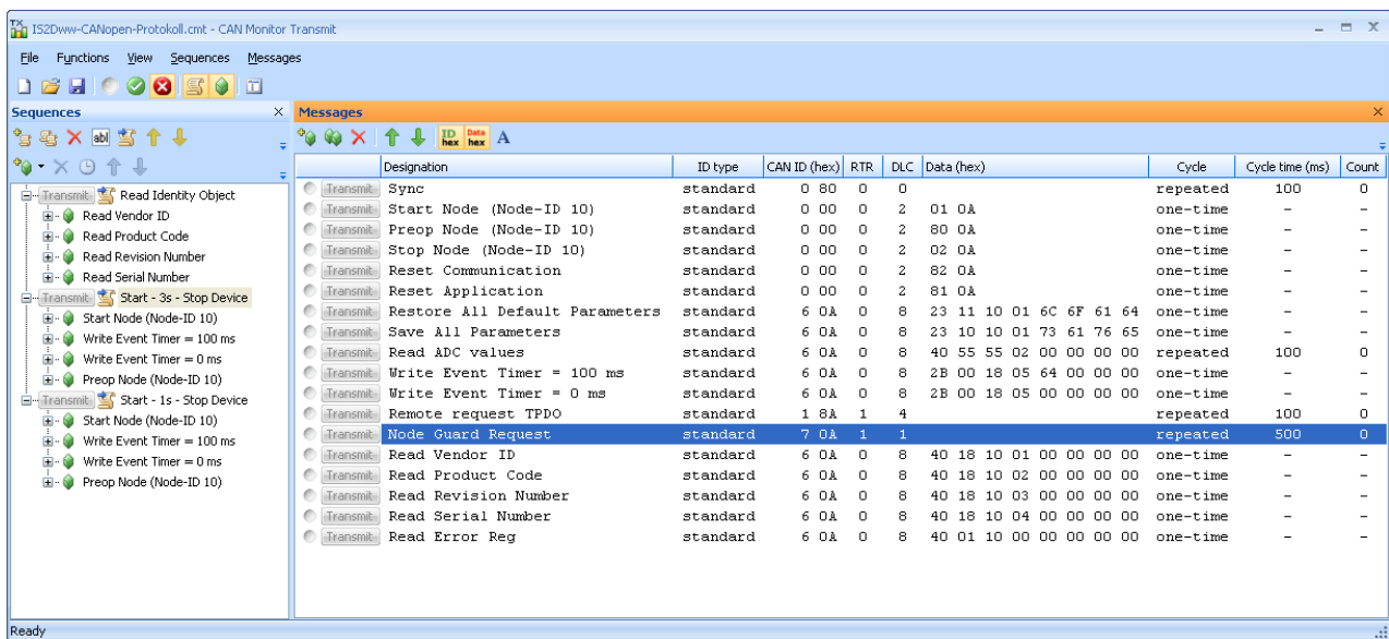
Figure 18: CAN Monitor Transmit
